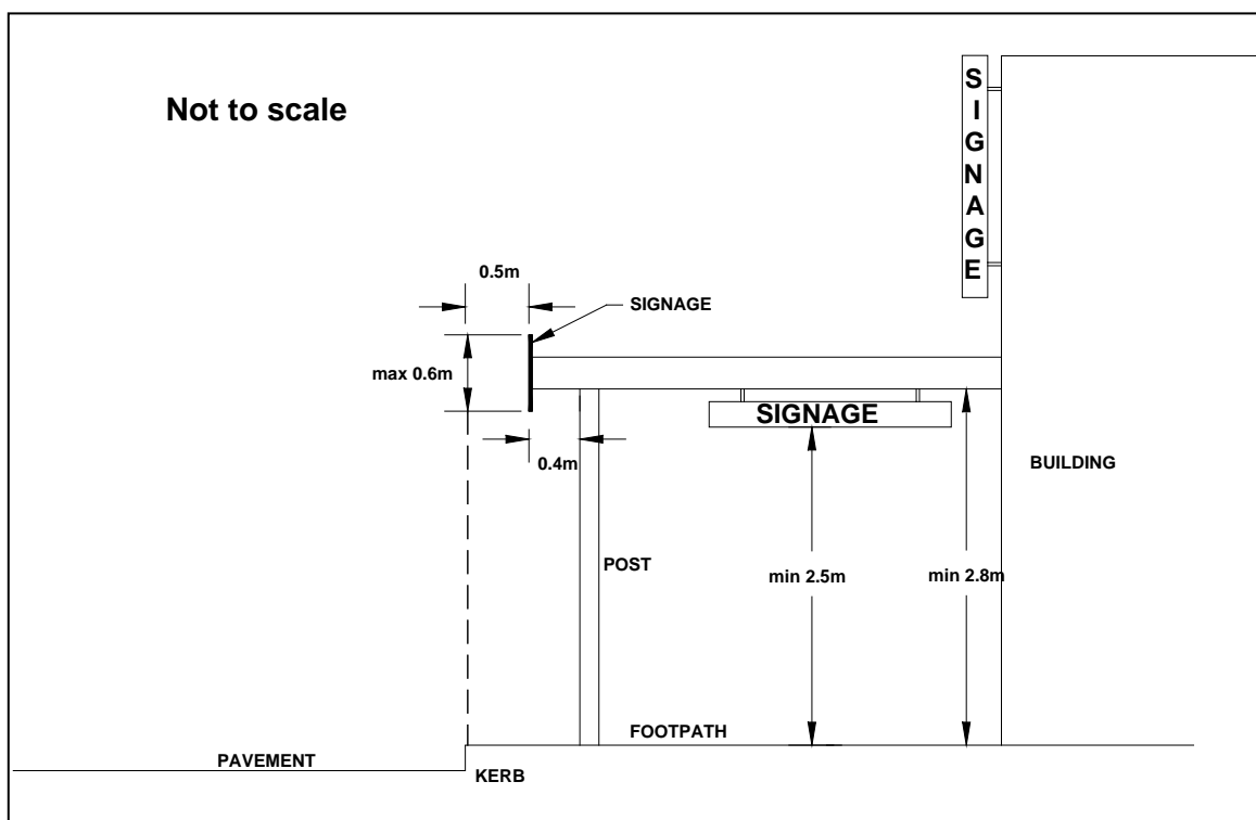
Figure 3.3 – Verandah Details
